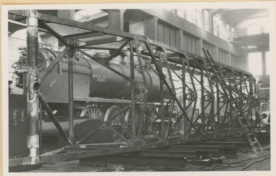
welded frame
