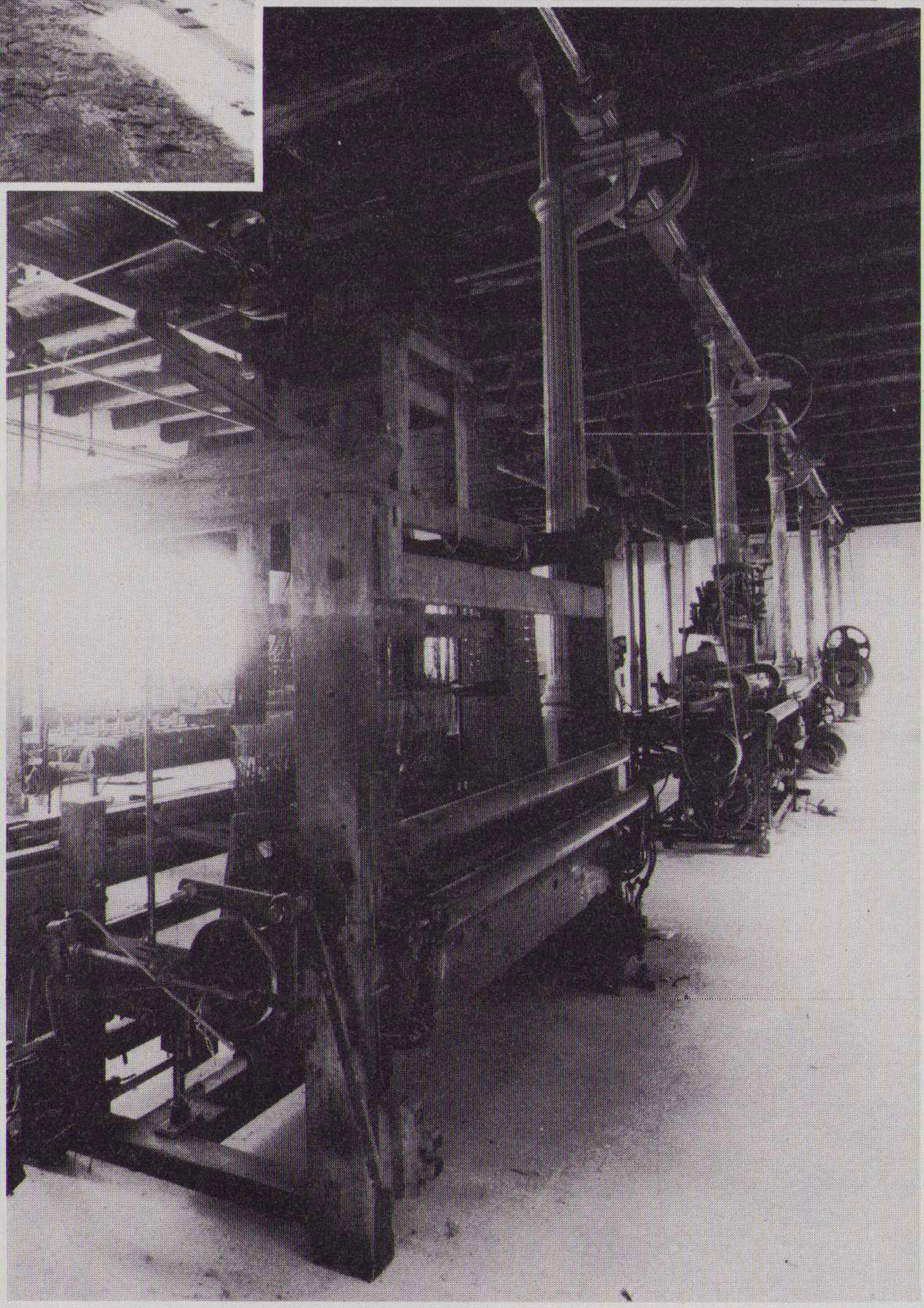
Jacquard-Webstuhl an Transmission.
